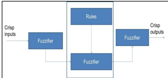
Fig 1: Fuzzy Topsis
